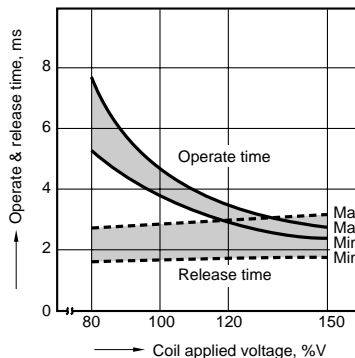
3-(2). Operate & release time (1 Form C type)
