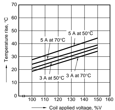
4-(1). Coil temperature rise (1 Form A type)
